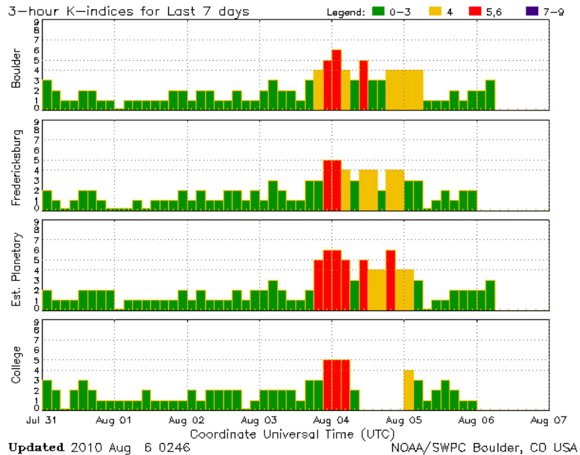
Multi-spectral solar image: http://sdo.gsfc.nasa.gov/data/ K-Indices from http://www.swpc.noaa.gov/alerts/k-index.html
