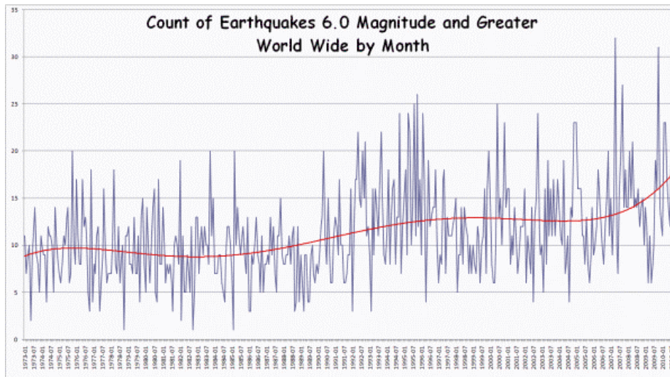
Graphs of worldwide Earthquakes 1973 to current 2010 from http://urbansurvival.com/week.htm
