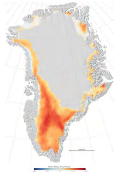
The Special Sensor Microwave Imaging radiometer was used to create this image of the 2007 Greenland melting anomaly which reflects the difference between the number of melting days occurring in 2007 and the average number of melting days during the period 1988 to 2006. -- from NASA/Earth Observatory
