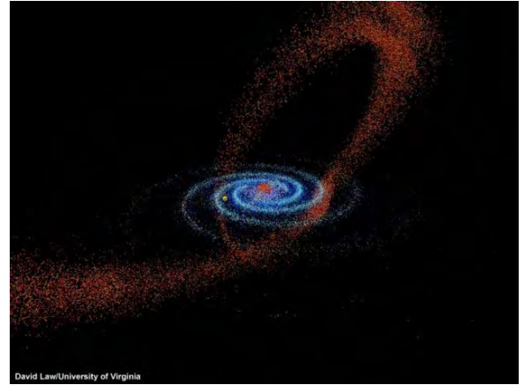
Computer generated map (2003) by David Law at the University of Virginia showing this Solar System (yellow dot) to be near the intersection of a portion of the Milky Way and a portion of Sagittarius Galaxy.
